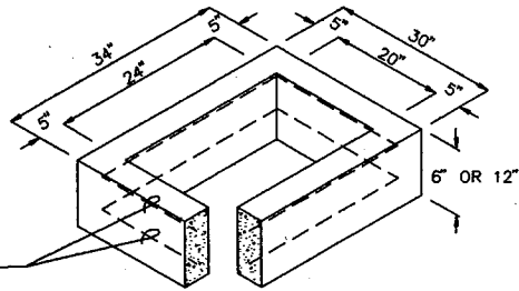
RISER SECTION
