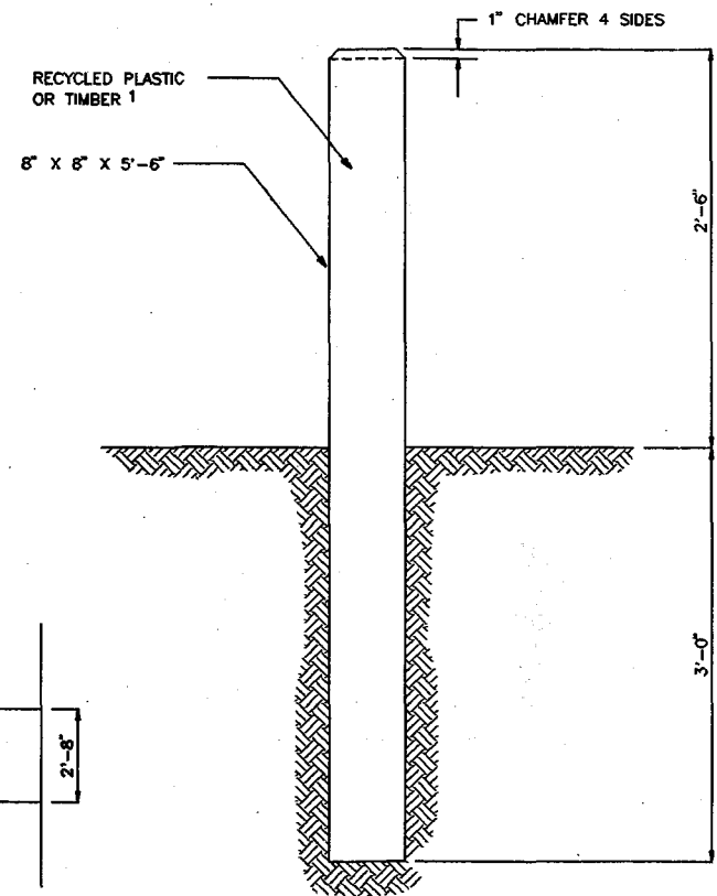
FIXED BOLLARD
