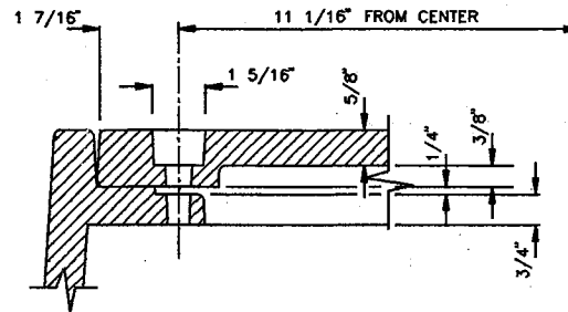
BOLT-DOWN DETAIL
