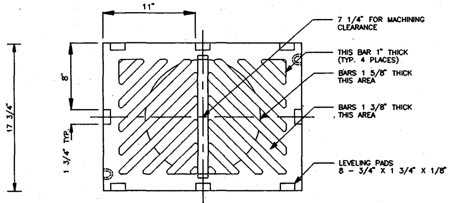
BOTTOM VIEW
