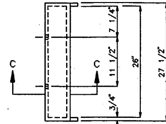
HOOD DETAIL
