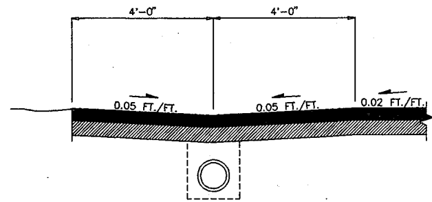
TURNPIKE SHOULDER
