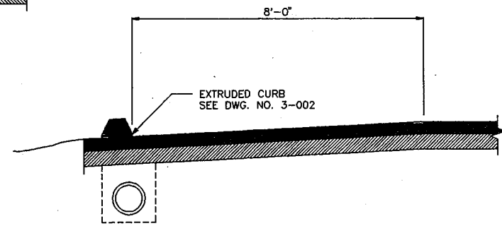
CURBED SHOULDER
