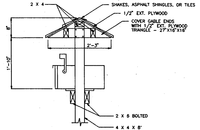
DETAIL
