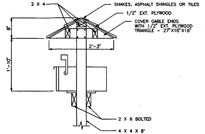
DETAIL
