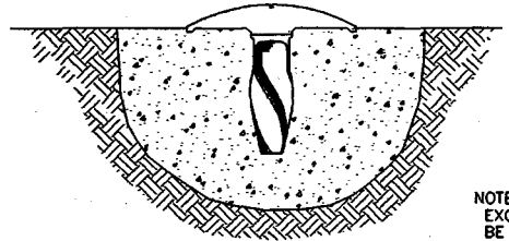
LEDGE ROCK OR CONCRETE INSTALLATION
