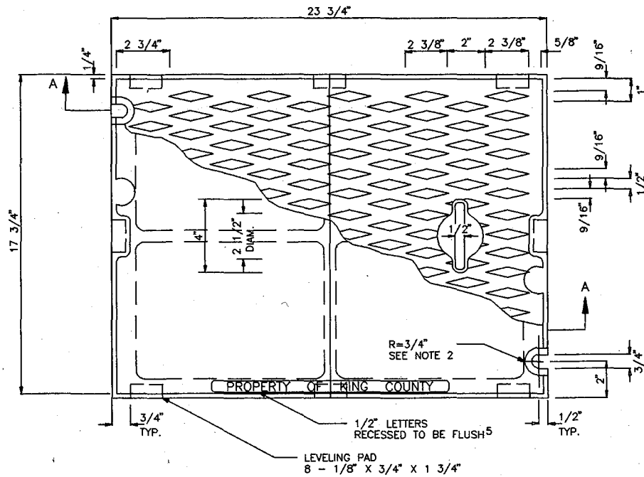
PLAN COVER
