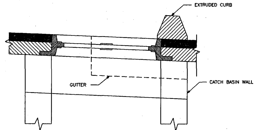
EXTRUDED CURB
