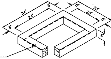
6" RISER SECTION
