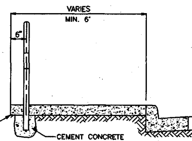
CEMENT CONCRETE
