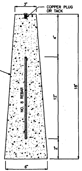
SECTION B-B
