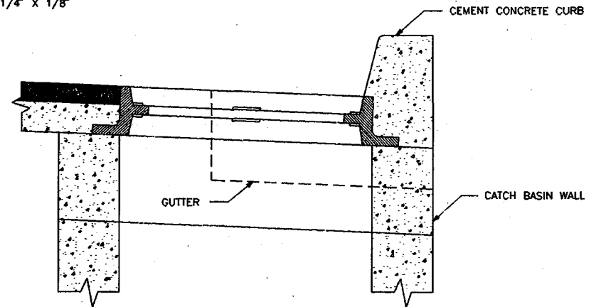
VERTICAL CURB
